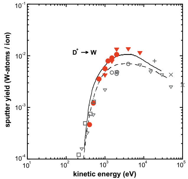
Fig. 3. Total sputter yields of polycrystalline tungsten bombarded by \text{D}^+ ions. Full (red) symbols have been obtained within this work; (circles represent bombardment on e-beam evaporated and triangles on magnetron sputter deposited W films); the dashed line represents recent TRIM.SP calculations [12], while the solid line shows earlier TRIM.SP predictions [18]. Previously published data are included for comparison: ( \nabla ) [15], ( \circ ) [18], (squares) [19], (+) [20] and (x) [18]. (For interpretation of the references to color in this figure legend, the reader is referred to the web version of this article).
