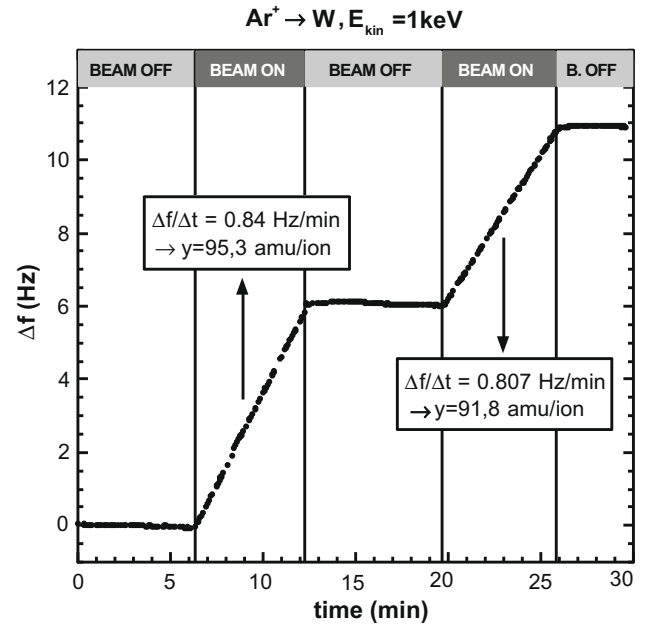
Fig. 1. Typical frequency response of the QCM to irradiation of the W film by Ar + ions. Two subsequent measurements are shown.
