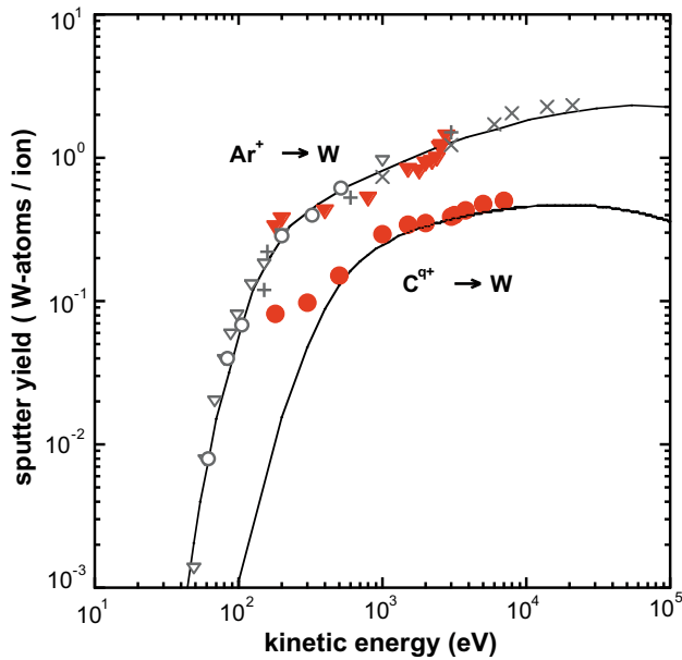
Fig. 2. Total sputter yields of polycrystalline tungsten bombarded by \text{Ar}^+ and \text{C}^{9+} ions. Full (red) symbols have been obtained within this work; solid lines represent TRIM.SP calculations [12]. Previously published data are included for comparison: ( \nabla ) [13], ( \circ ) [14], (+) [15] and (x) [16]. (For interpretation of the references to color in this figure legend, the reader is referred to the web version of this article).
