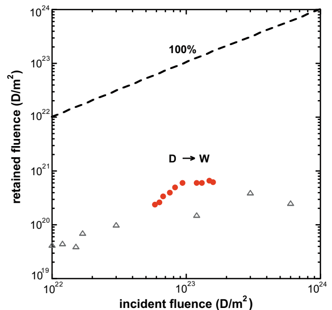
Fig. 4. Deuterium retention in polycrystalline tungsten under bombardment by 100 eV \text{D}^+ . The dashed line represents a hypothetical absolute retention of all incoming flux. Full (red) symbols have been obtained within this work, while open triangles are implantation data reported in [21]. (For interpretation of the references to color in this figure legend, the reader is referred to the web version of this article).
